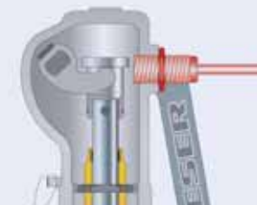
Lift indicator J39: Adaptor for lift indicator H4 J93: Lift indicator
