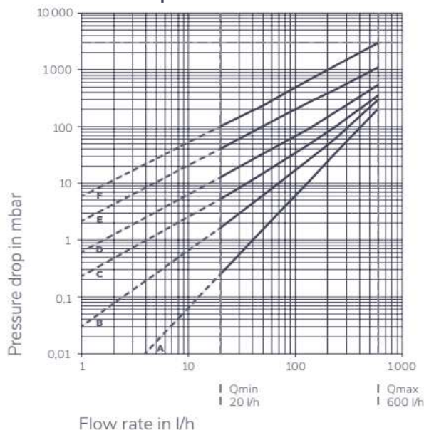
DN15 Pressure Drop
