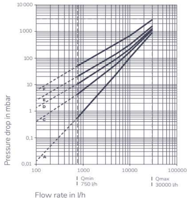
DN50 Pressure Drop
