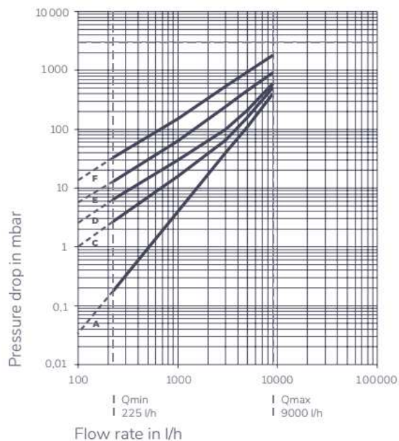
DN40 Pressure Drop
